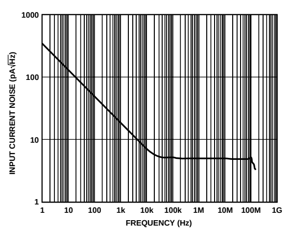
Figure 51. Input Current Noise vs. Frequency ( \overline{DISENABLE} = +V_S )
