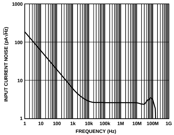
Figure 48. Input Current Noise vs. Frequency ( \overline{DISENABLE} = \text{Open} )
