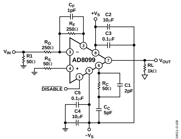
Figure 62. Amplifier Configuration for CSP Package, Gain = -1
