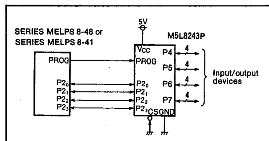
Fig.1 Basic connection
