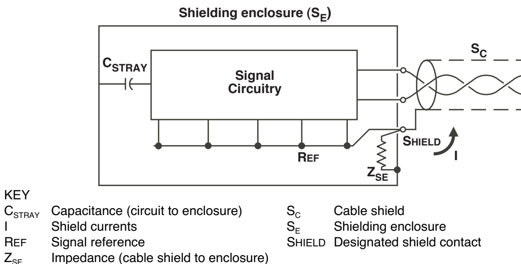
Figure B2 – Common-impedance coupling (i) (Pin 1 problem)
