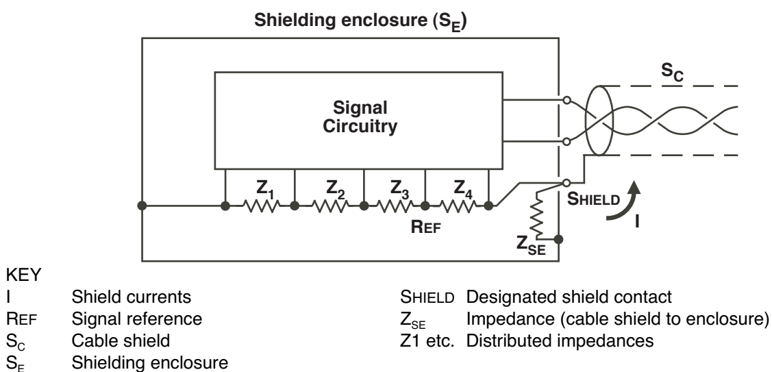
Figure B3 – Common-impedance coupling (ii)
