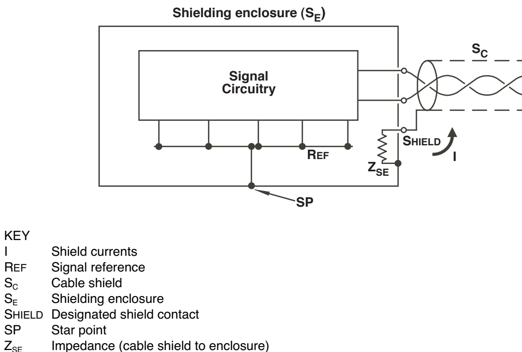
Figure B1 – Effects of the impedance of the connection between the cable shield and the enclosure
