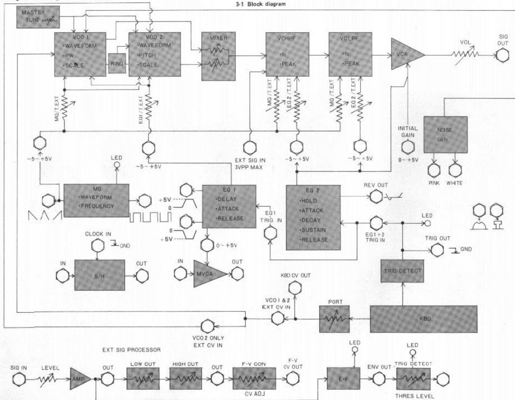
3-1 Block diagram
