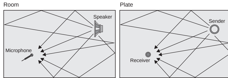
Fig. 4.3: Room reflections and reverb plate reflections
