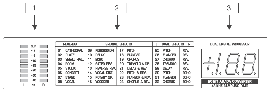
Fig. 1.2: Display section of the DSP1000P
